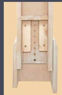
No. 210 MDF rear view of plinth base showing adjustable height feature. Plinth is removable to lower height more.
